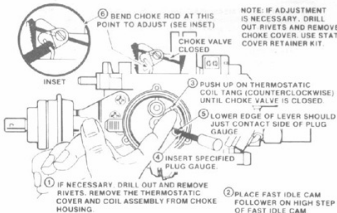
FIG. 3 CHOKE COIL LEVER ADJUSTMENT (See Note)
