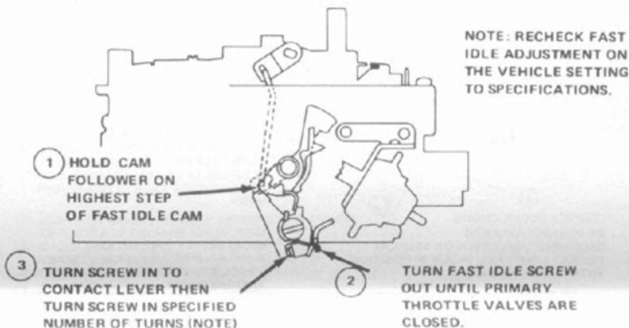
FIG. 4 FAST IDLE ADJUSTMENT (BENCH SETTING)
