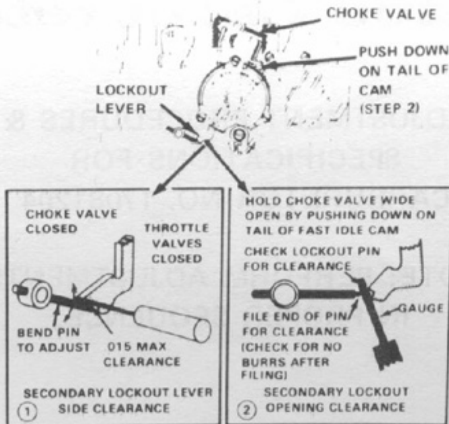
FIG. 12 SECONDARY LOCKOUT ADJUSTMENT
