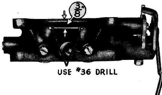
FIG. 1 - DRILL TWO HOLES WITH NO. 36 DRILL. PUT ONE HOLE DIRECTLY INTO EACH BARREL OF THE CARBURETOR.
