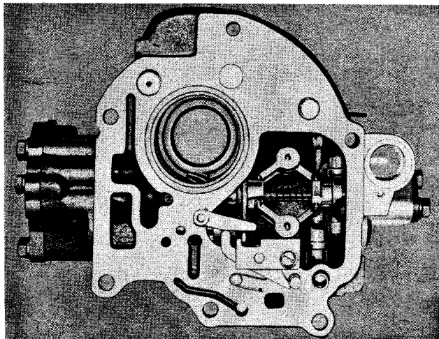
FIG. 3 - TO ELIMINATE PART-THROTTLE DOWNSHIFT, INSTALL EXTENSION CASE ASSEMBLY AS FURNISHED BY YOUR PARTS DEPOT AS SHOWN IN PHOTO ABOVE.
