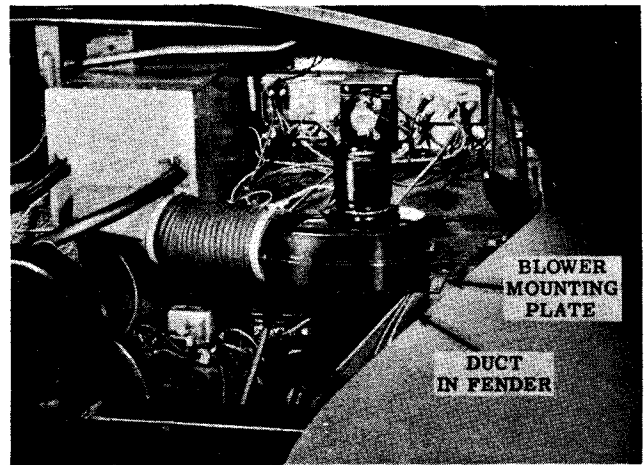
FIG.6 - NEW TRUCK CLIMATIZER INSTALLED
